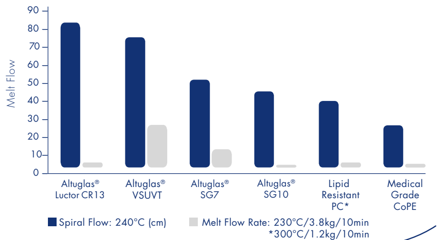
Chart 8: Melt Flow of Altuglas® & Altuglas® Luctor CR13
